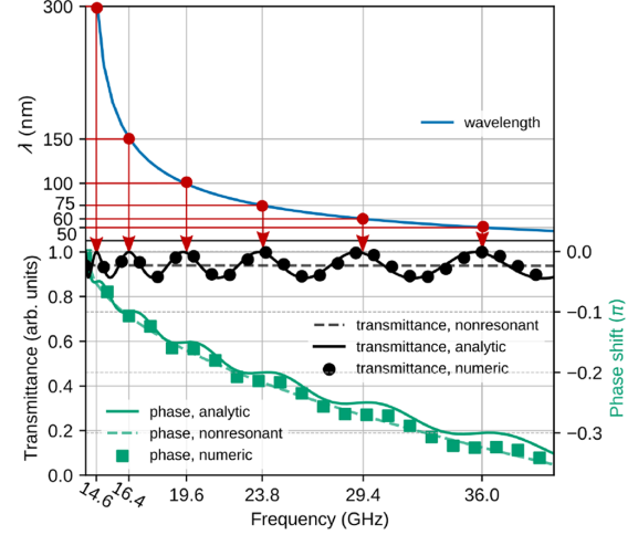
FIG. 3. SWs' wavelength (blue color) as a function of frequency. Red dots indicate fulfilled resonant conditions by Eq. (10). Enhancement of transmittance at these frequencies can be observed. Values on the horizontal axis represent the resonant frequencies. The transmittance (black color) and the phase shift (green color) for SWs traveling through the 150-nm-wide slab with respect to the frequency. Dots and squares represent the values obtained in the numerical simulations, while the solid lines represent the analytical results. Dashed lines represent the case when the reflection in the system is neglected. The value of the external field is equal to 0.5 T, reduced M_S in the slab is equal to 800 kA/m and reduced A_{\text{ex}} to 20 pJ/m.
