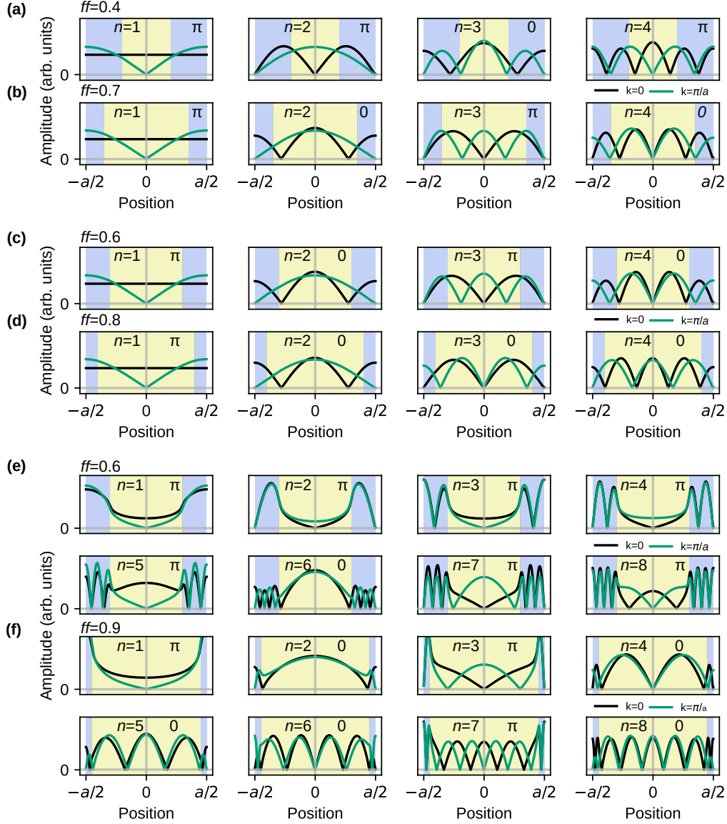
Figure 2. The SW's profiles |m_{\perp}| within the unit cell at the edges of BZ. Black line is calculated for k = 0 , green line for k = \pi/a . The values of the SW profiles and their derivatives allow determining the Zak phase for the band. (a) Results for ff = 0.4 . For n = 1 , n = 2 and n = 4 modes have different derivatives in the middle of unit cells, that suggest value of Zak phase equal to \pi . For n = 3 Zak phase is equal to 0. (b) Results for ff = 0.7 . For n = 1 and n = 3 Zak phase is equal \pi , and for n = 2 and n = 4 Zak phase is equal 0. (c) Results for ff = 0.6 . For n = 1 and n = 3 Zak phase equal to \pi . For n = 2 and n = 4 Zak phase is equal to 0. (d) Results for ff = 0.8 . Only for n = 1 Zak phase is equal \pi , everywhere else is equal to 0. For exchange-dipolar waves, 8 SW's profiles are presented. (e) Results for ff = 0.6 . For n = 1, n = 2, n = 3, n = 4, n = 5, n = 8 Zak phase is equal to \pi , everywhere else is equal to 0. (f) Results for ff = 0.9 . For n = 1, n = 3, n = 7 Zak phase is equal to \pi , everywhere else is equal to 0.
