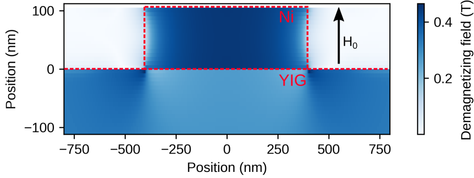
Fig. 2.5 The distribution of static demagnetizing field (out-of-plane component) for the structure composed of the uniform film made of yttrium-iron-garnet (YIG) and Ni strip, placed on the top. The following material parameters were assumed: YIG layer ( M_{S,YIG} = 143 kA/m, \lambda_{ex,YIG} = 14.5 nm), Ni strip ( M_{S,Ni} = 480 kA/m, \lambda_{ex,Ni} = 7.7 nm). YIG layer and Ni strip have the same thickness 112 nm. The width of the strip is 800 nm. An external magnetic field of the value 0.5 T is applied along the vertical axis, saturating the magnetization in the out-of-plane direction.
