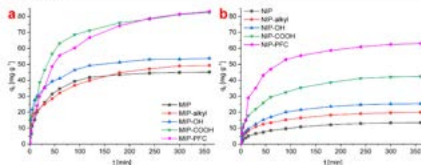
Figure 4. Kinetic plots for PFOS adsorption on (a) MIPs and (b) NIPs, conducted in aqueous solution at an initial PFOS concentration of 0.1 mg mL -1 .
