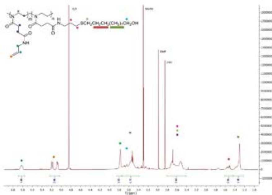
Figure S3. ^1\text{H} NMR spectrum of poly(AllylamidOx)-OH measured in \text{CD}_3\text{OD} .
