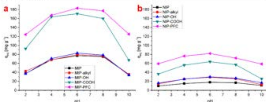
Figure 5. Influence of pH on PFOS adsorption by (a) MIPs, (b) NIPs, conducted in aqueous solution at an initial PFOS concentration of 0.1 mg mL -1 .
