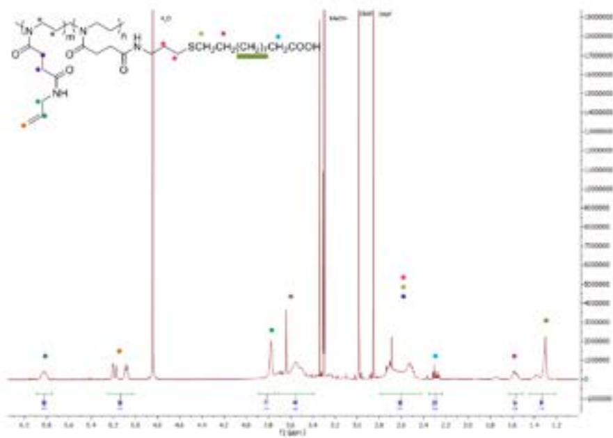
Figure S4. 1 H NMR spectrum of poly(AllylamidOx)-COOH measured in CD 3 OD.
