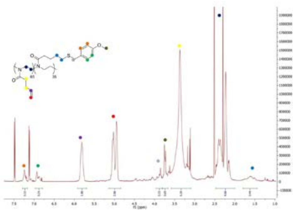
Figure S2. ^1\text{H} NMR spectrum of poly(ButenOx)-4MBM.
