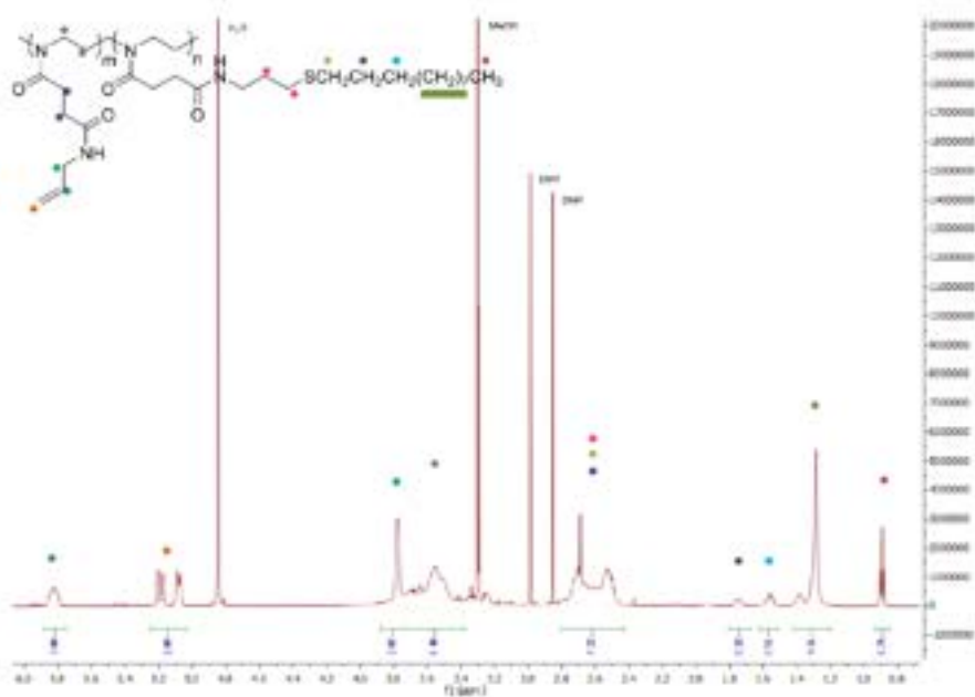
Figure S2. ^1\text{H} NMR spectrum of poly(AllylamidOx)-alkyl measured in \text{CD}_3\text{OD} .
