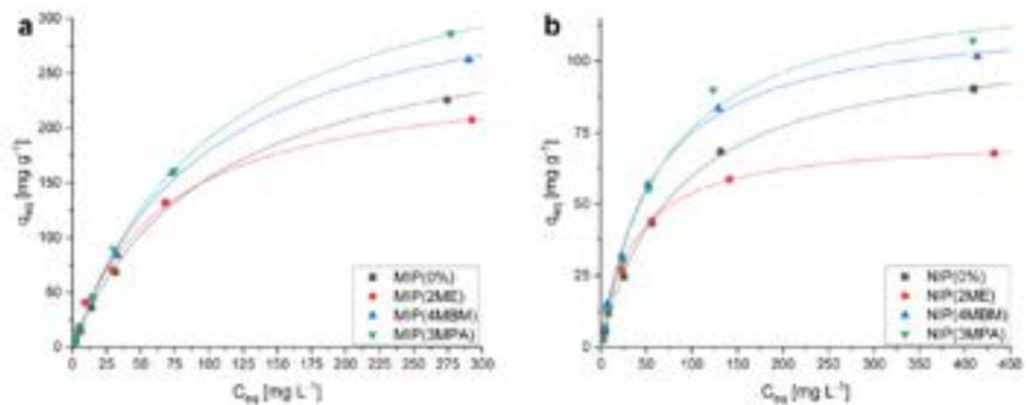
Figure S9. Adsorption isotherms of PrP adsorption from methanol solutions on (a) MIPs and (b) NIPs.
