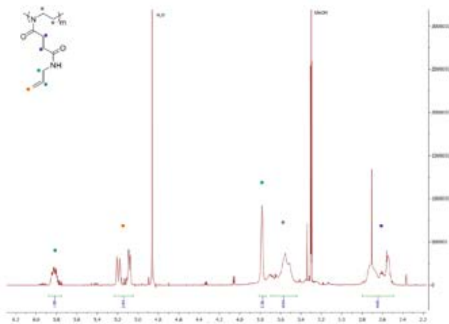
Figure S1. 1 H NMR spectrum of poly(AllylamidOx) measured in CD 3 OD.
